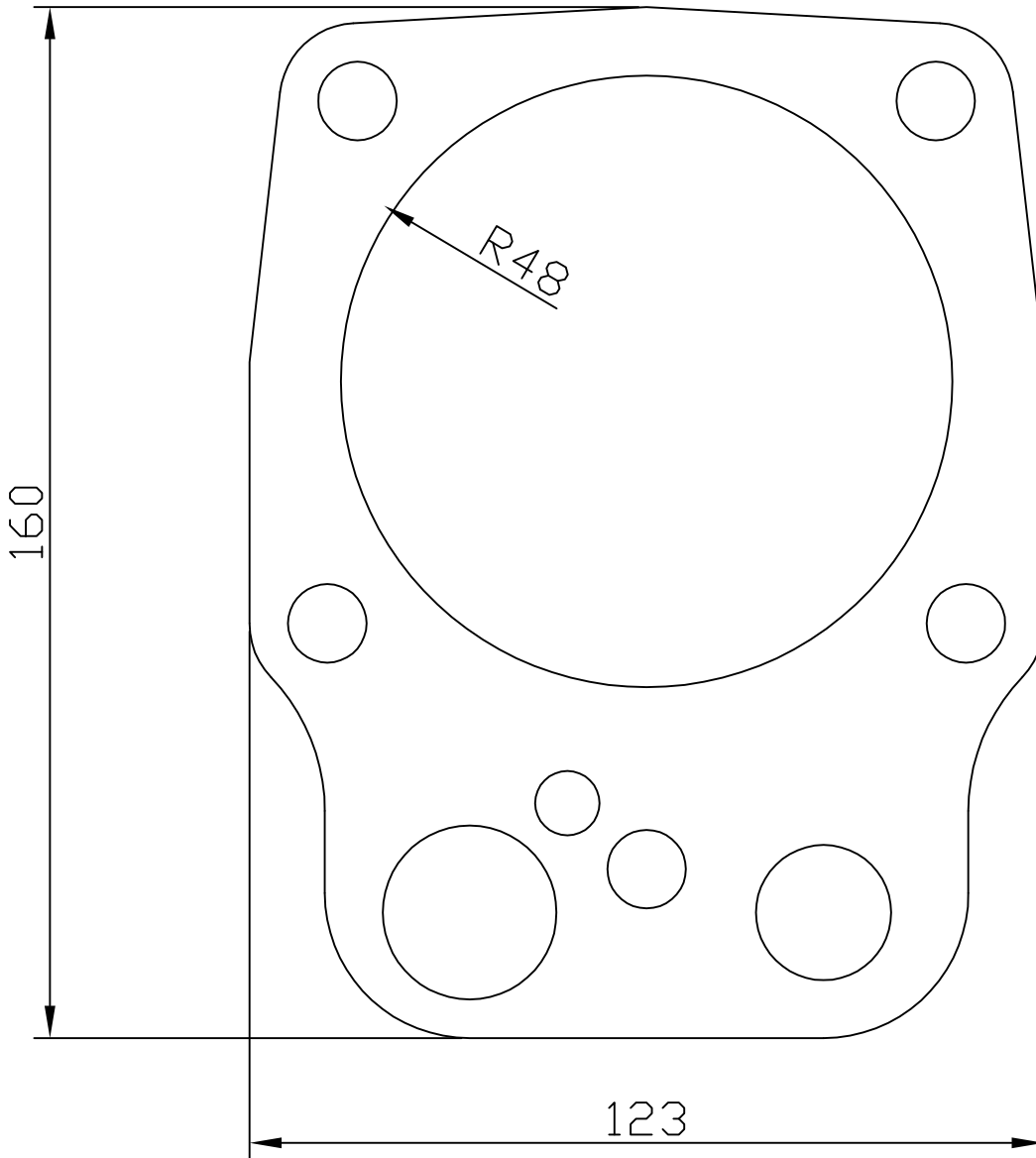
BSA M20 Cylinder Base Gasket R1
